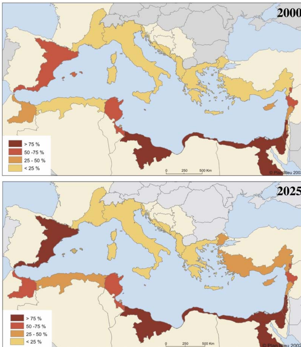
Figure 2: Exploitation Indices of Renewable Natural Water Resources
